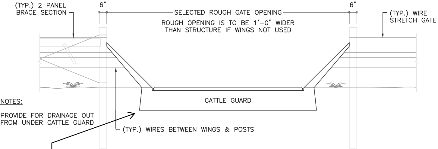
TYPICAL CATTLE GUARD N.T.S.
