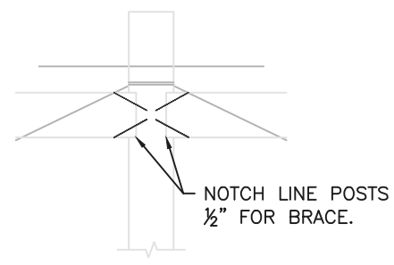
POST JOINT — DETAIL N.T.S.
