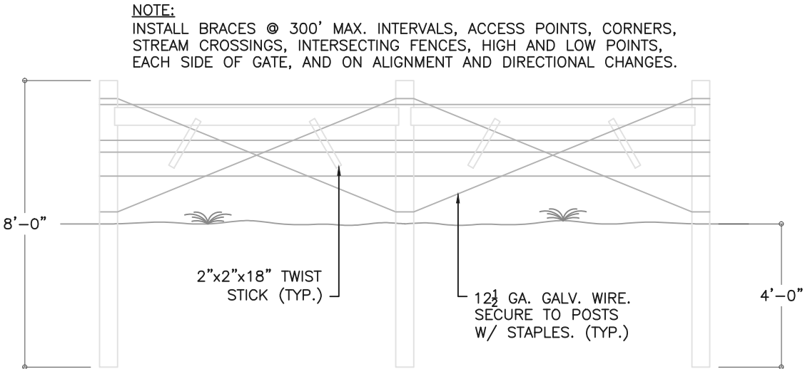
TYPICAL 2 PANEL BRACE SECTION N.T.S.
