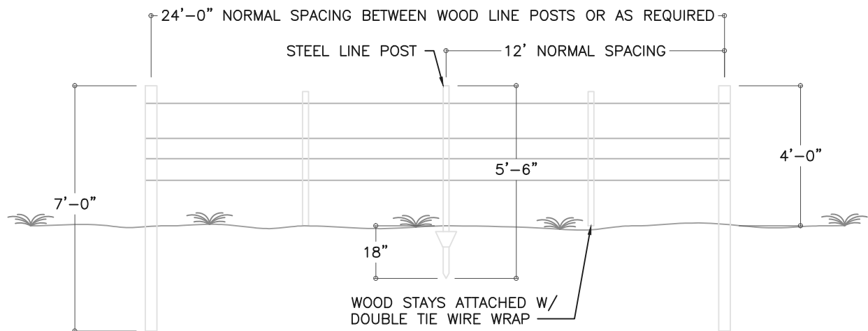
TYPICAL LINE SECTION N.T.S.
