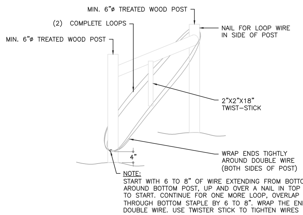
BRACE SECTION WIRING — DETAIL N.T.S.
